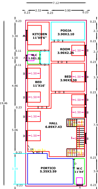
GROUND FLOOR RESIDENTIAL PLAN
