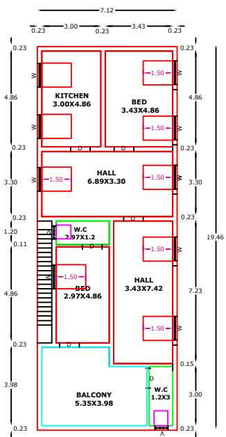
FIRST FLOOR RESIDENTIAL PLAN
