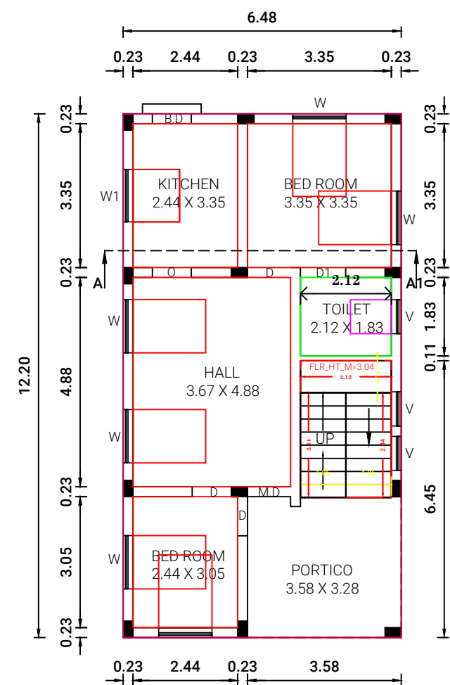
PLAN - GROUND FLOOR (PROPOSED)
