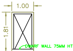
WICKET GATE
