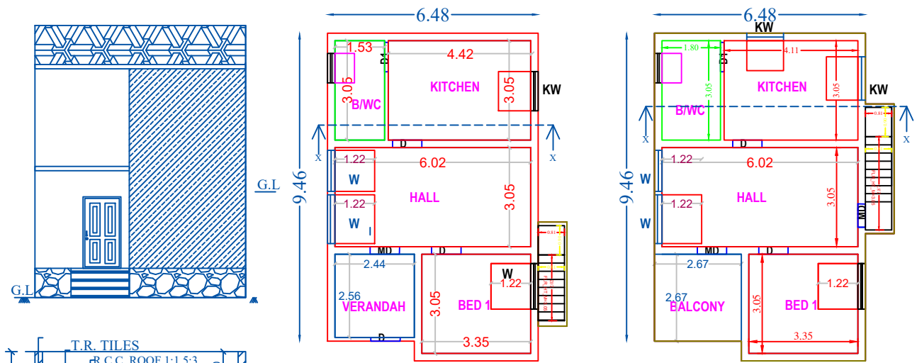
PLAN - GROUND FLOOR (EXISTING) PLAN - FIRST FLOOR (PROPOSED)
