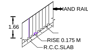
STAIRCASE
