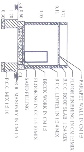
SECTION ON "A-A"
