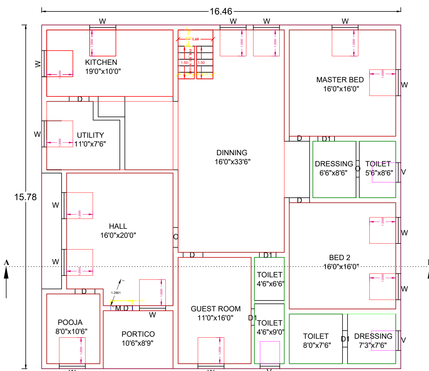
GROUND FLOOR
