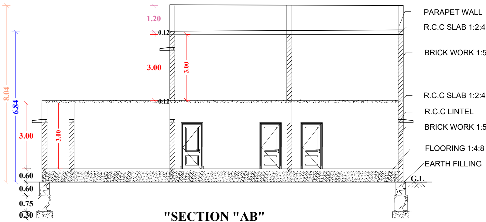
"SECTION "AB"
