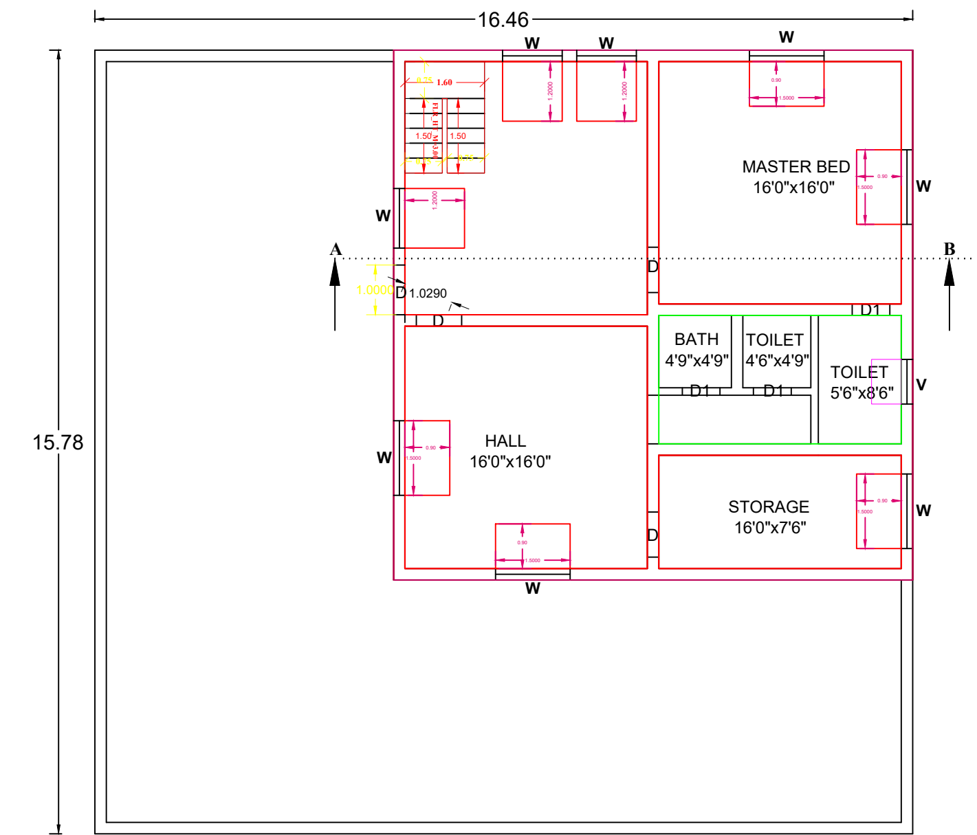
FIRST FLOOR
