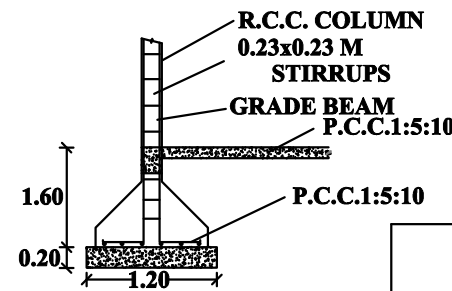
COLUMN DETAIL
