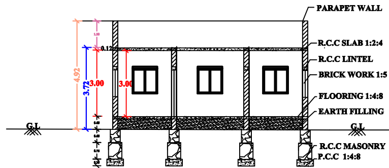
"SECTION "AB"
