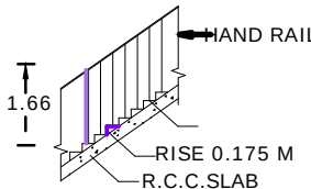
STAIRCASE
