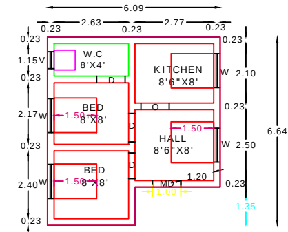
GROUND FLOOR RESIDENTIAL PLAN
