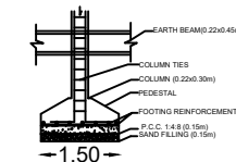
FOUNDATION DETAILS
