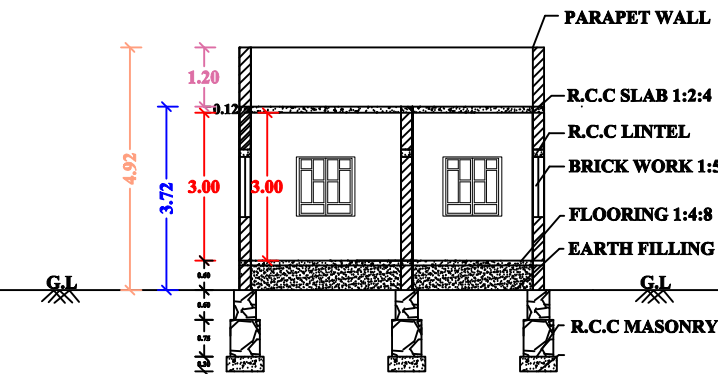
"SECTION "AB"
