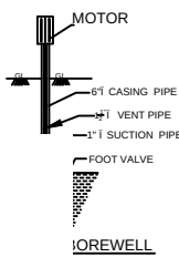
BOREWELL
