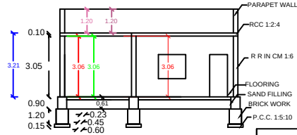
SECTION AB
