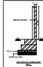
SECTION AB
