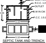
SEPTIC TANK AND TRENCH
