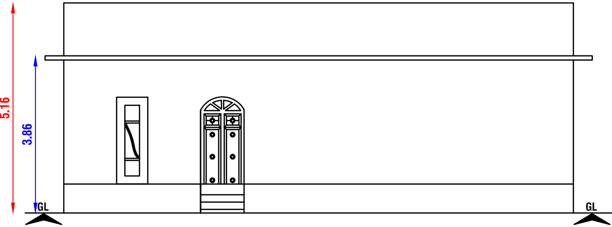
FRONT ELEVATION
