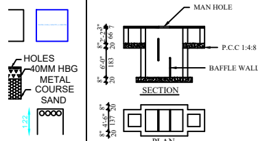
SEPTIC-TANK DETAIL
