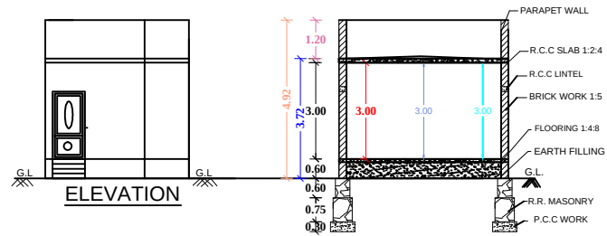
CROSS SECTION
