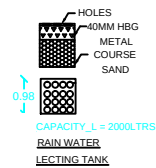
CROSS SECTION
