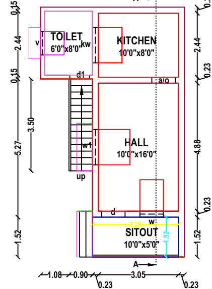
PLAN - GROUND FLOOR RESIDENCE
