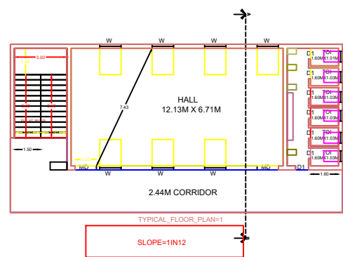
PRO.GROUND FLOOR PLAN
