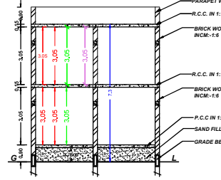
SECTION "AB"
