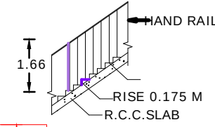
STAIRCASE
