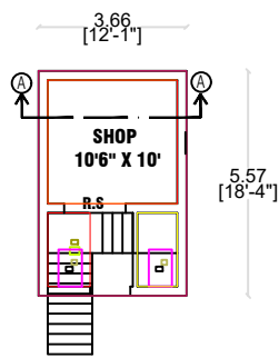
PROPOSED FIRST FLOOR PLAN
