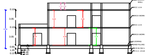
SECTION AB
