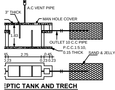
SEPTIC TANK AND TRECH
