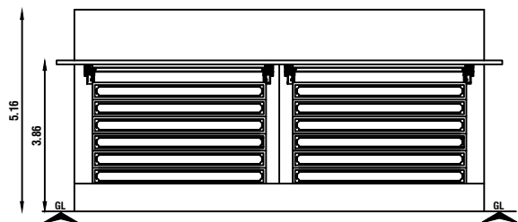
FRONT ELEVATION
