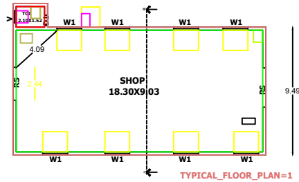
TYPICAL_FLOOR_PLAN=1
