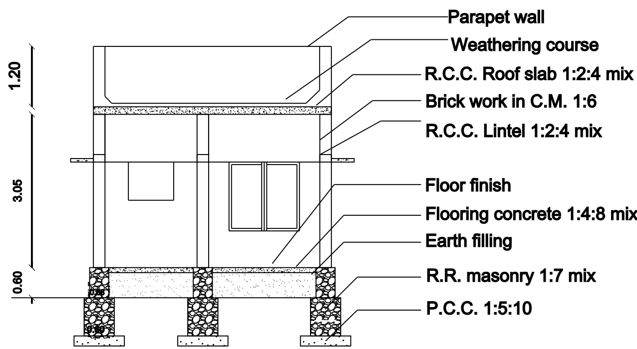
SECTION AB
