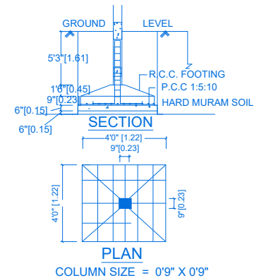
FOUNDATION DETAILS
