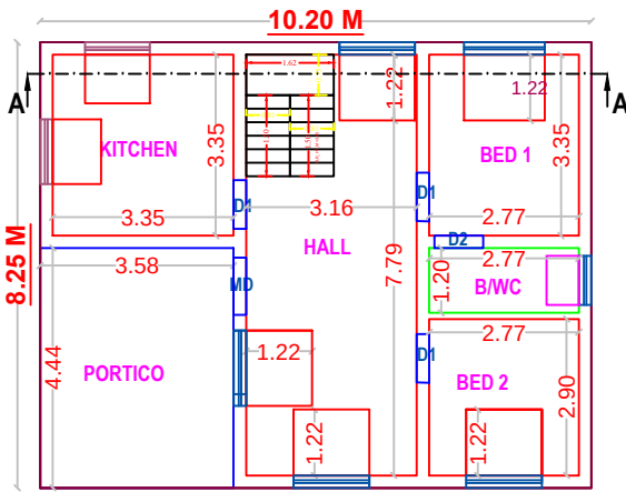
PLAN - GROUND FLOOR (PROPOSED)
