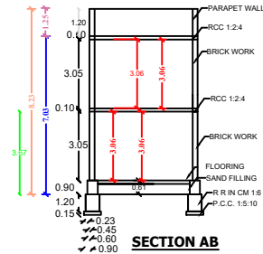
SECTION AB
