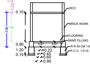
SECTION AB
