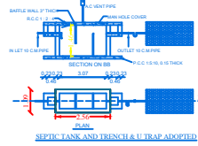
SEPTIC TANK AND TRENCH & U-TRAP ADAPTED
