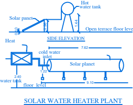
SOLAR WATER HEATER PLANT
