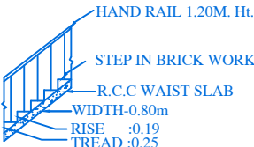
STAIR DETAIL
