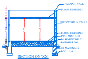
SECTION ON 'XX'
