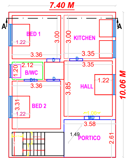
PLAN - GROUND FLOOR ( EXG. BUILDING )
