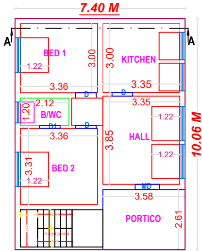
PLAN - FIRST FLOOR ( PROPOSED )
