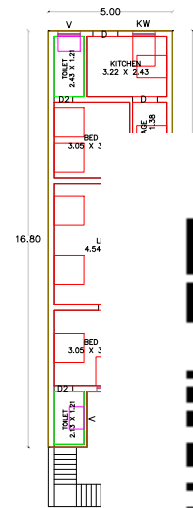
PLAN - Gf ( PRG )
