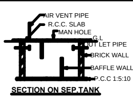
SECTION ON SEP. TANK
