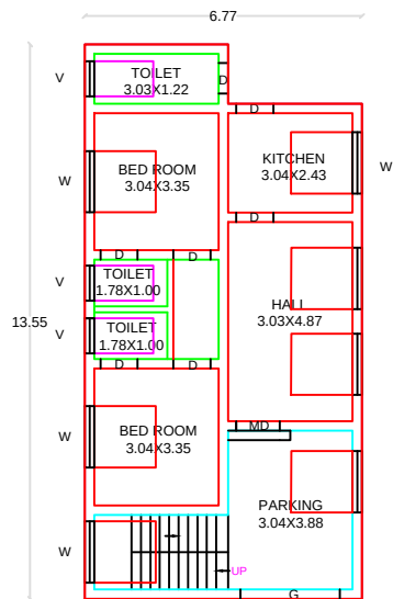
PROPOSED GF PLAN
