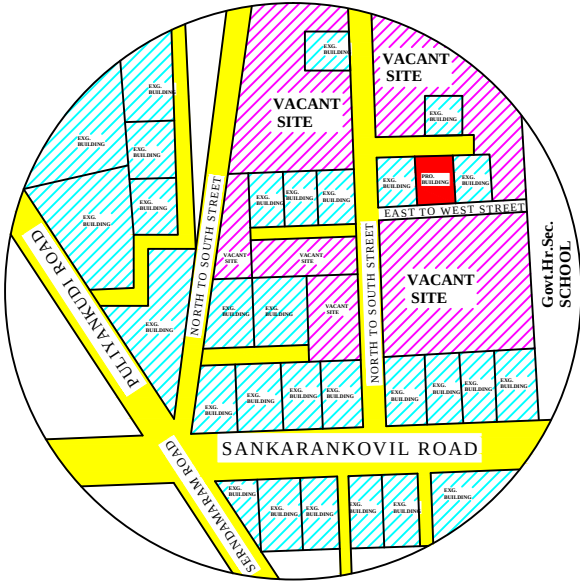
TOPO PLAN
