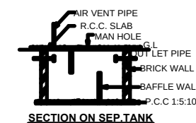
SECTION ON SEP.TANK
