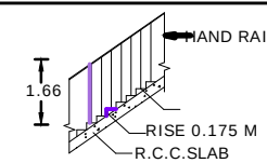
STAIRCASE
