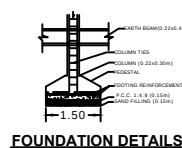
FOUNDATION DETAILS
