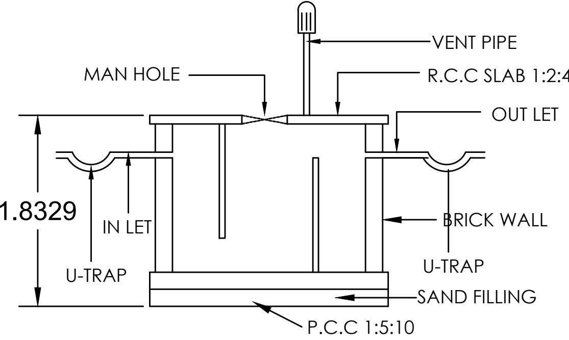
SECTION E,F SEPTIC TANK DETAIL
