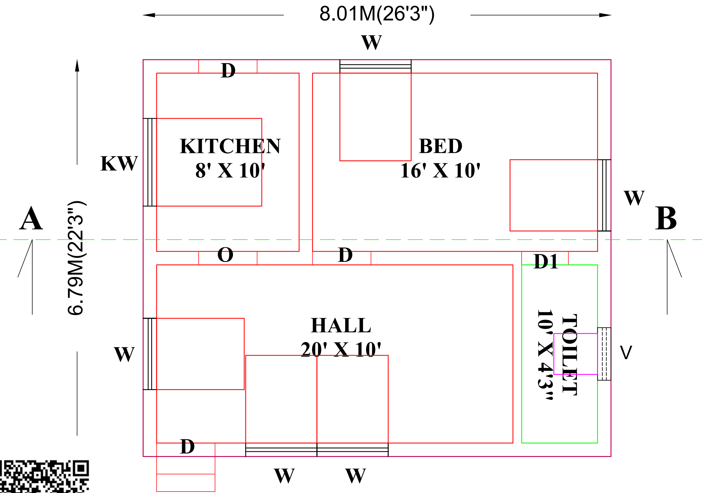
PLAN
