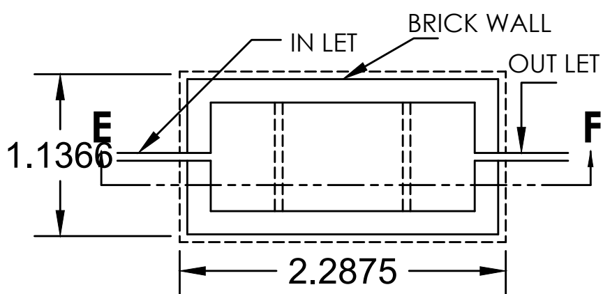
PLAN PLAN OF SEPTIC TANK
