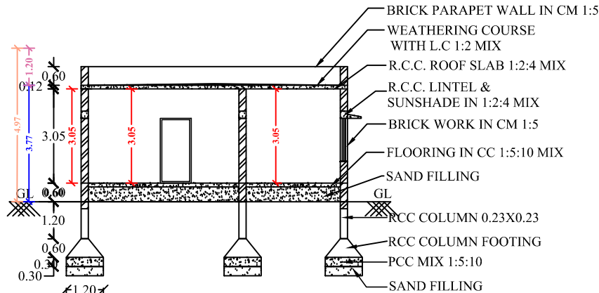
SECTION OF "BS"
