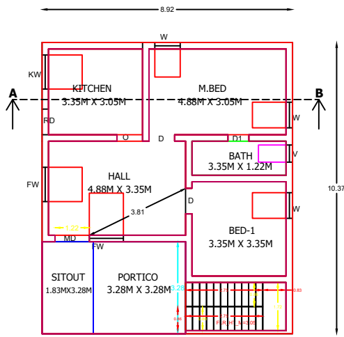
TYPICAL_FLOOR_PLAN=1,2
