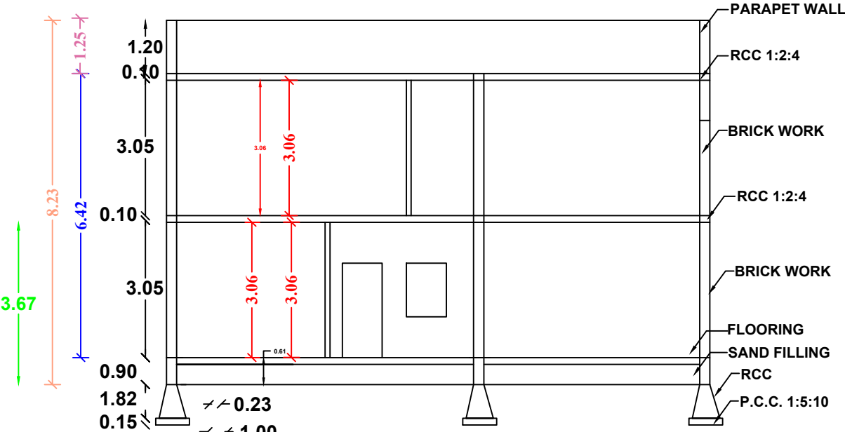
SECTION AB
