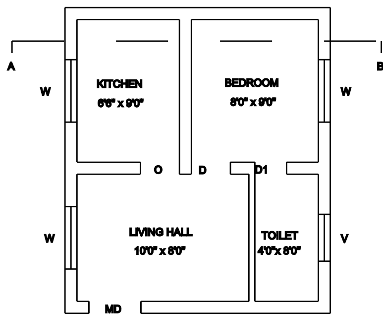
PLAN - GROUND FLOOR
