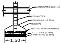
FOUNDATION DETAILS
