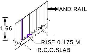
STAIRCASE
