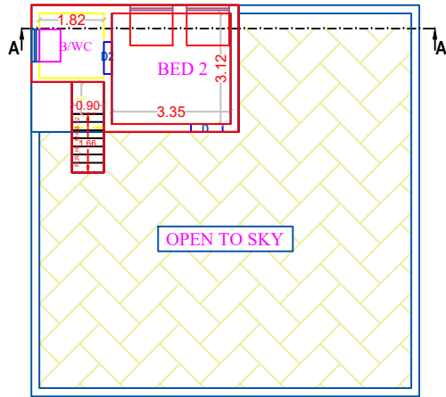
PLAN - FIRST FLOOR ( PROPOSED )
