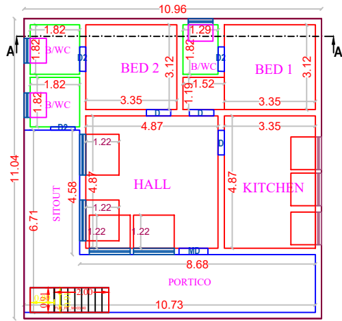
PLAN - GROUND FLOOR ( PROPOSED )
