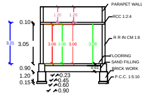
SECTION AB
