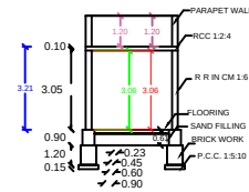
SECTION AB
