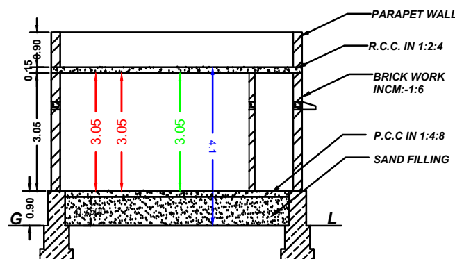
SECTION "AB"
