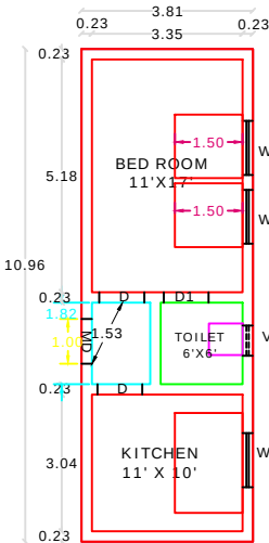
GROUND FLOOR RESIDENTIAL PLAN
