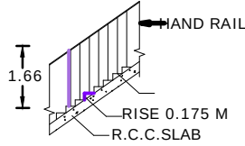
STAIRCASE
