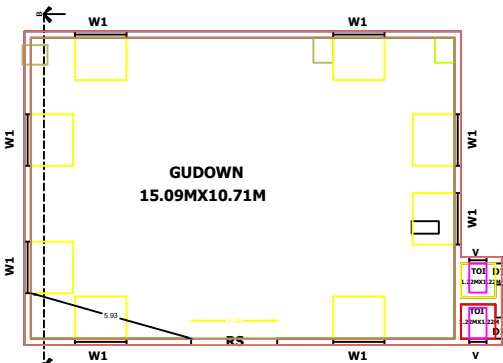
TYPICAL_FLOOR_PLAN=1
