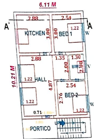
PLAN - GROUND FLOOR (PROPOSED - 671.45 SQ.FT.)
