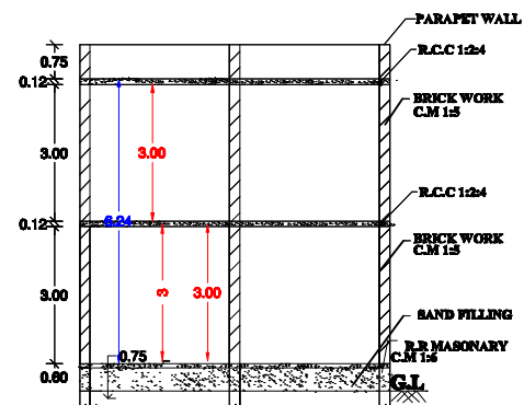
SECTION ON "BB"
