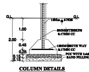
COLUMN DETAILS
